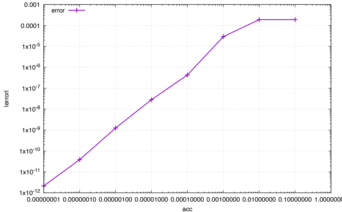
Error in erf(1) vs accuracy
